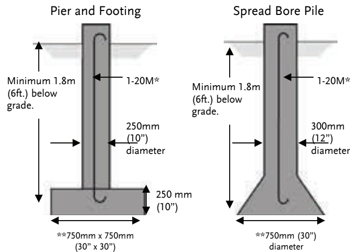
FIGURE 5—Piles or piers
