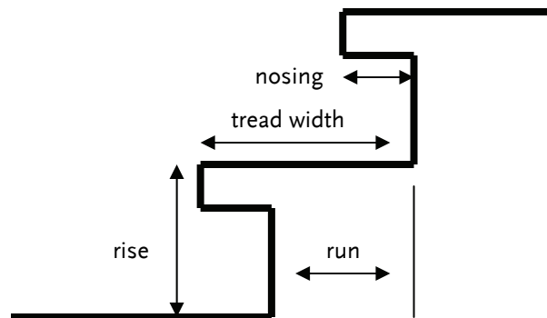
FIGURE 14—Stair Detail
