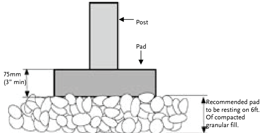
FIGURE 4—Surface Pad Foundation
