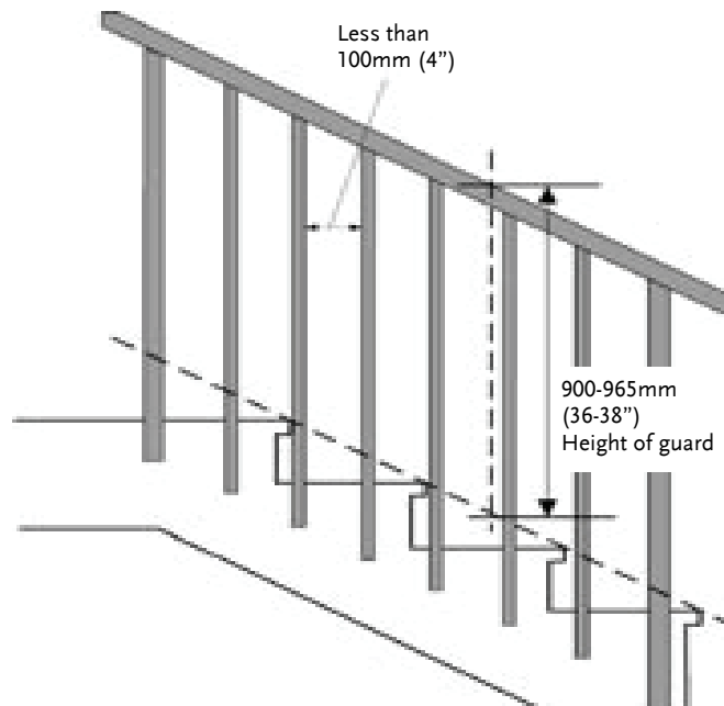
FIGURE 15—Combined Guardrail/Handrail
