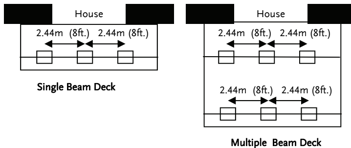
FIGURE 6—Deck Beam Spacing
