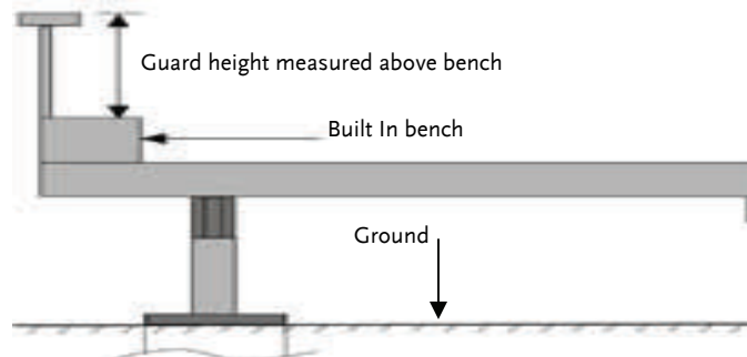
FIGURE 13- Guardrail and Bench
