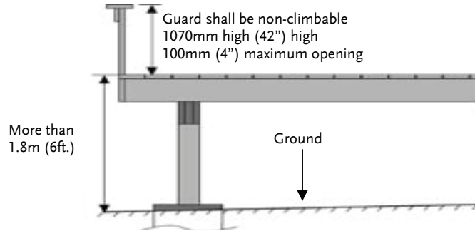
FIGURE 12—Guardrail Height
